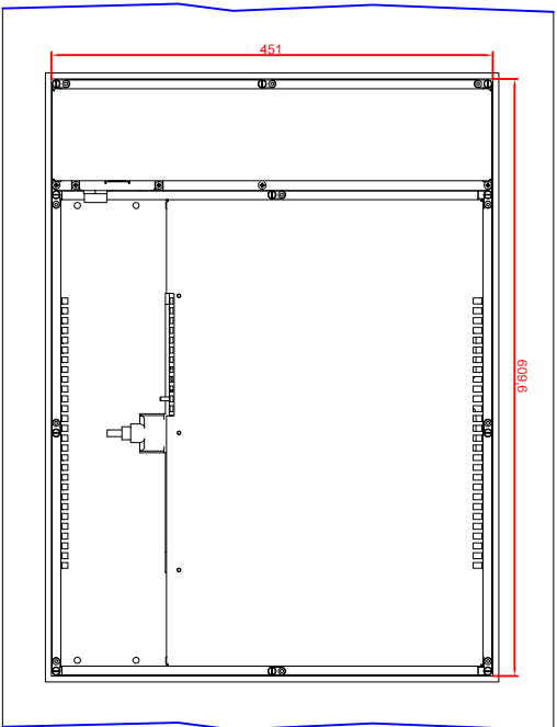
rear view with install measure
