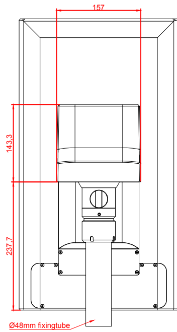
rear view
