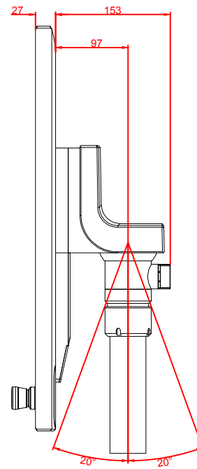
right view
