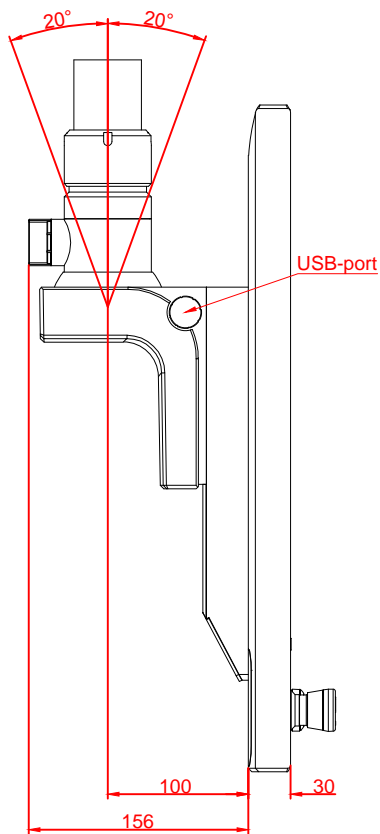
left view
