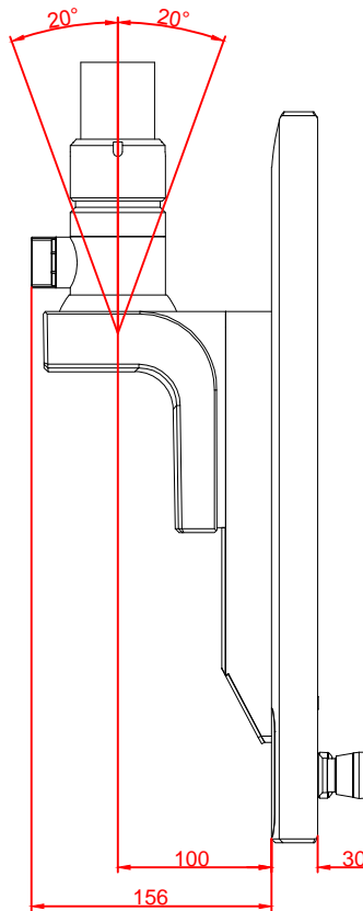
left view
