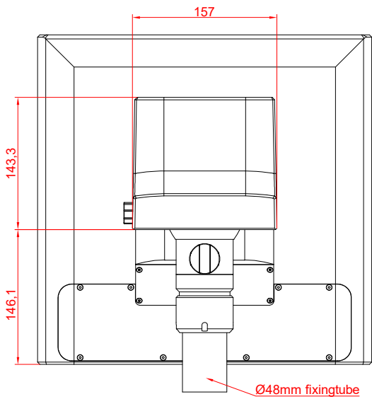
rear view
