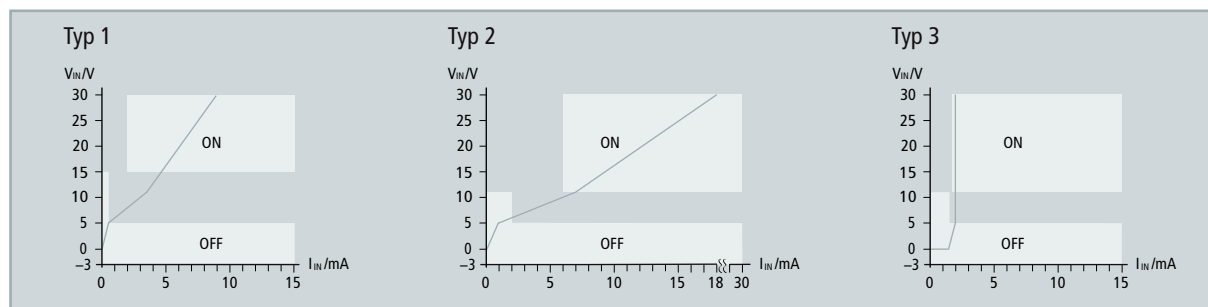
Fig. 3 Characteristic curves of the three types of input (24 V DC) from Beckhoff
