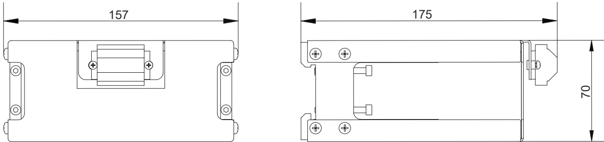
Fig. 4: C9900-U330_dimensions
