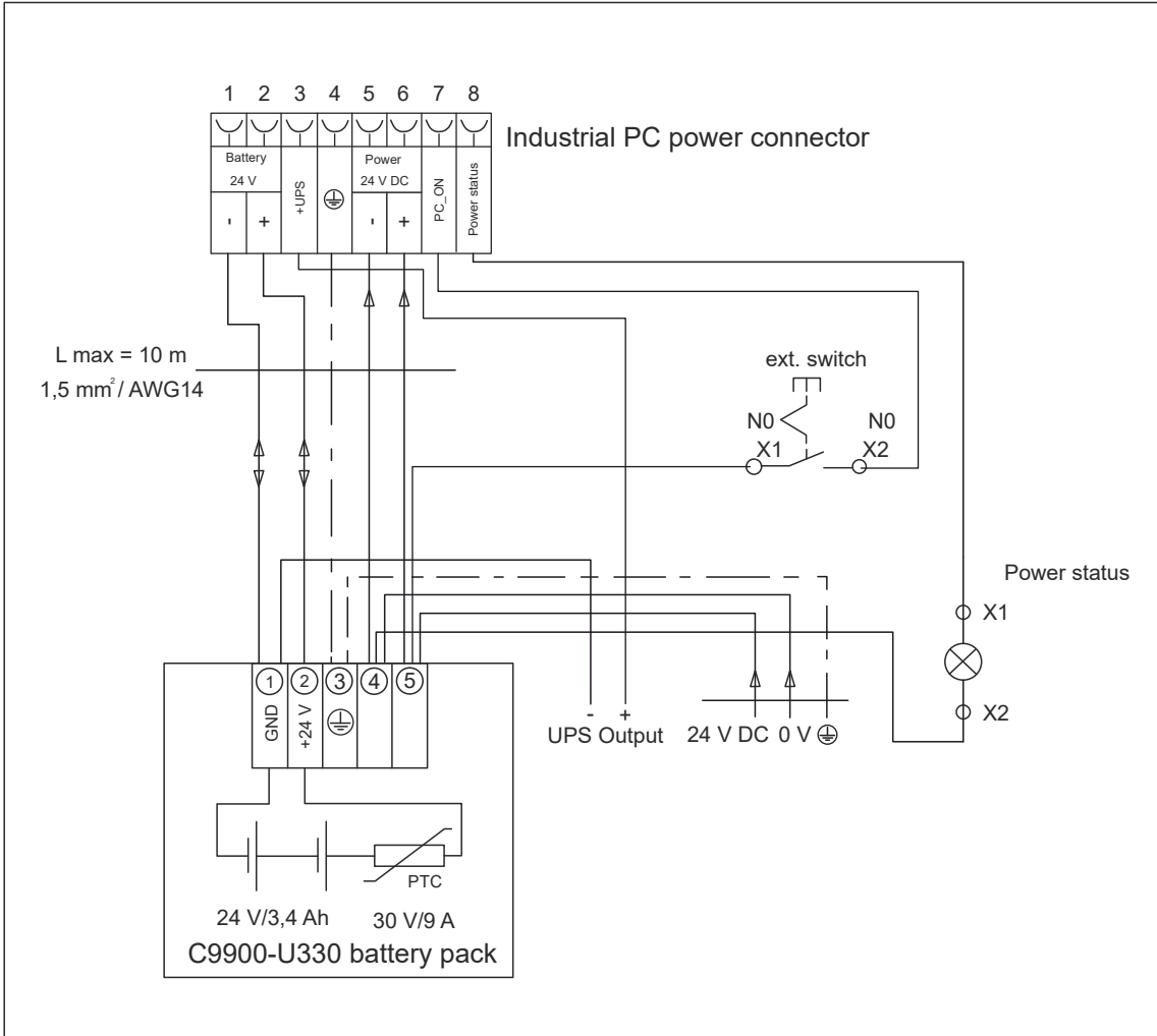
Fig. 8: C9900-U330_wiring diagram-8-pin
