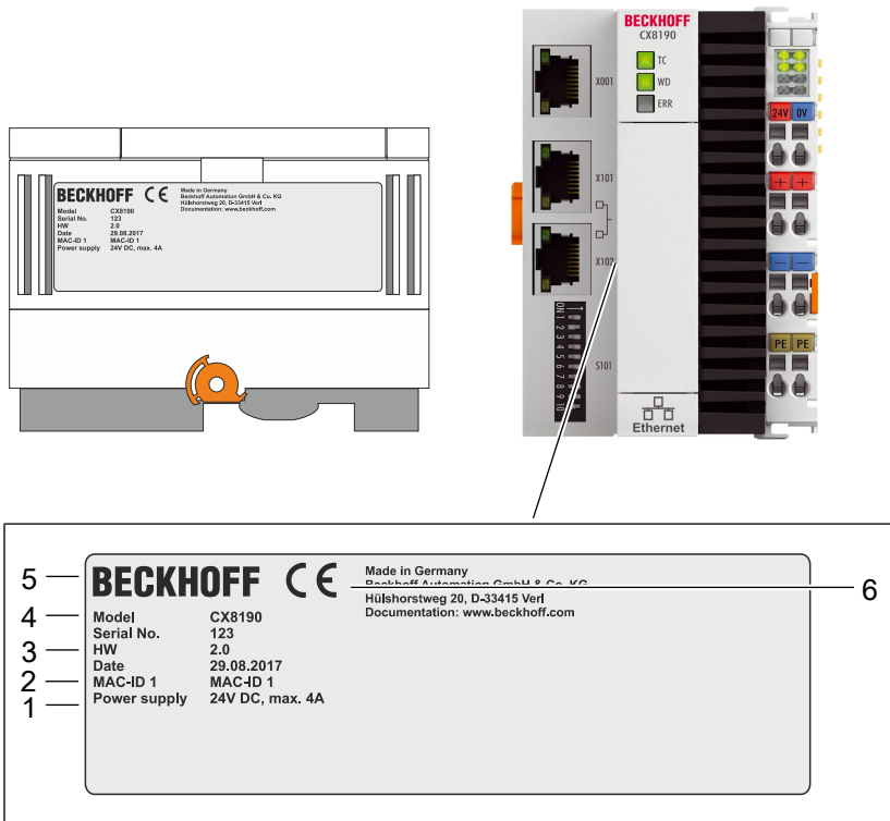
Abb. 2: CX8190 Typenschild.
